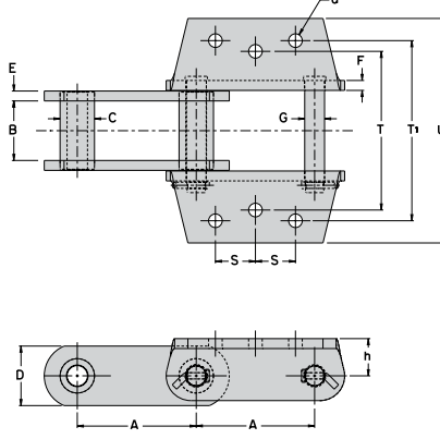
K-3 Attachment
