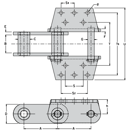
K-5 Attachment
