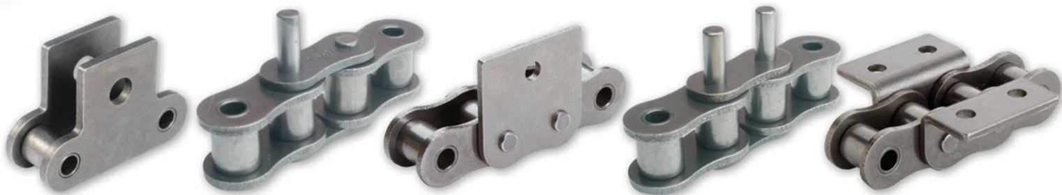
Laser-Cut Attachments and Custom Extended Pins
